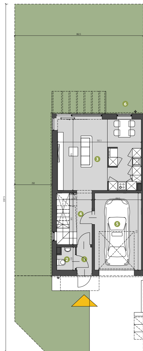
PARTER
